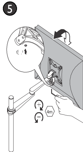
PROXIMA Clamp Mount Assembly
